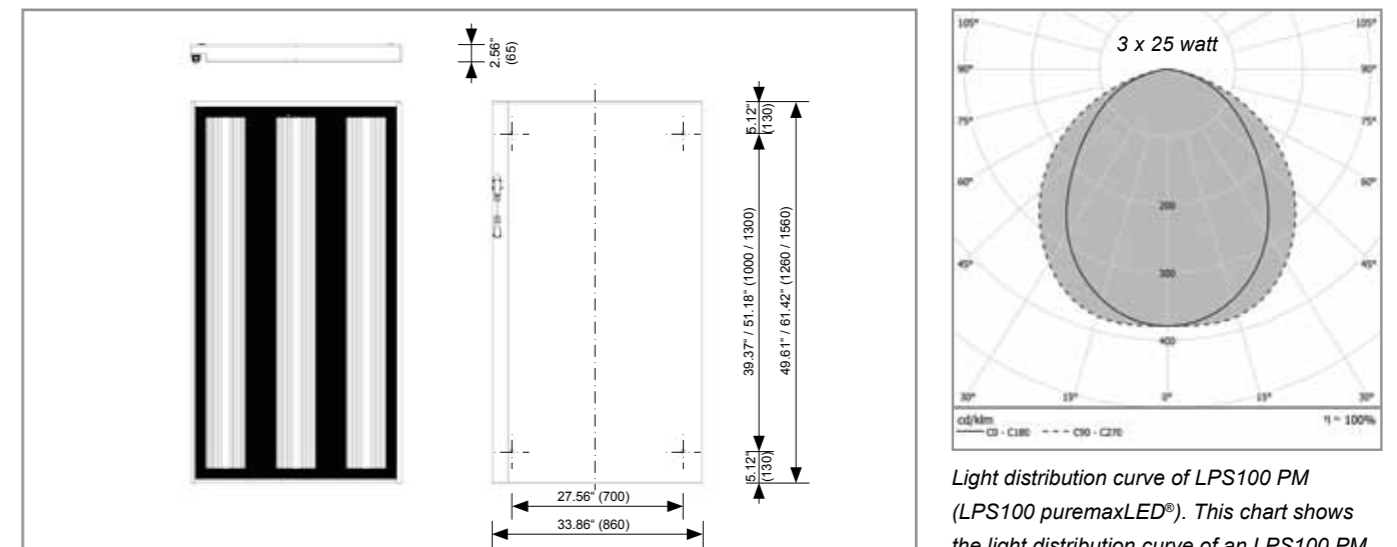
Exterior and mounting dimensions of the LPS100 PM. All data in Inches (mm).
