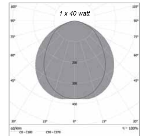
Light distribution curve of VAO PM (VAO puremaxLED). This chart shows the light distribution curve of a VAO PM with 1 x 40 watt.
