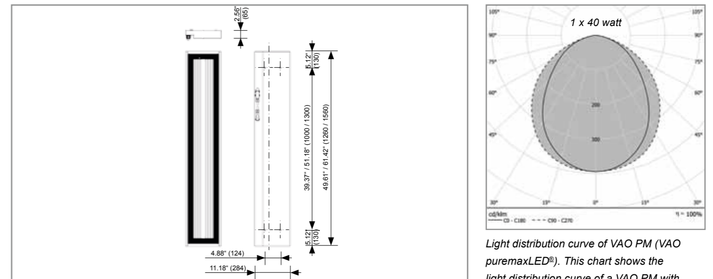
Exterior and mounting dimensions of the VAO PM. All data in Inches (mm).
