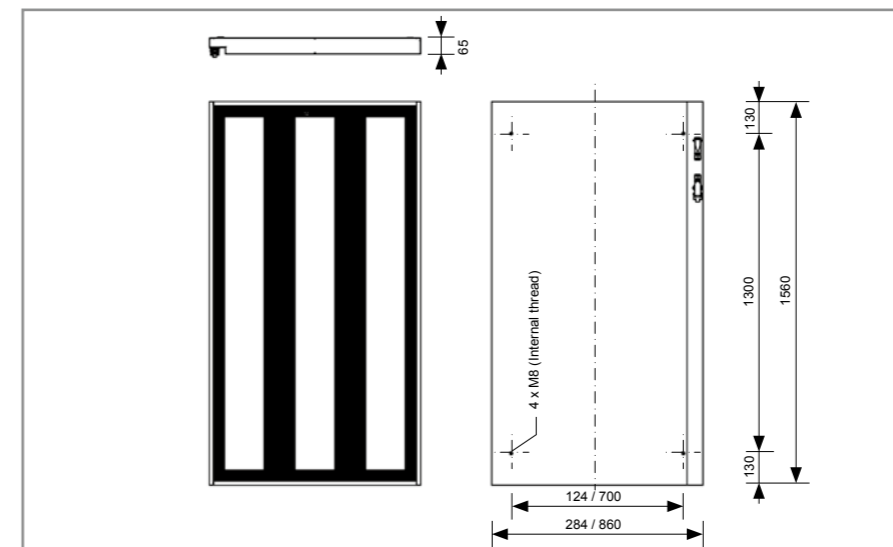
Exterior and mounting dimensions of the ARO PM. All data in mm.
