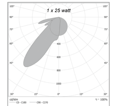
Light distribution curve of ARO PM (ARO puremaxLED®). This chart shows the light distribution curve of an ARO PM with 1 x 25 watt.
