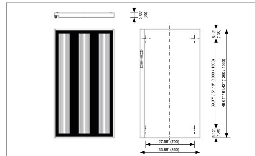
Exterior and mounting dimensions of the LPS100 PM. All data in Inches (mm).
