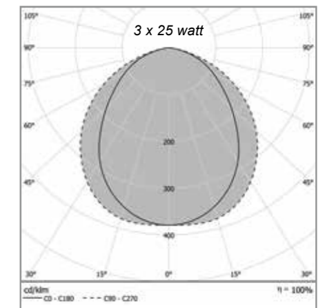
Light distribution curve of LPS100 PM (LPS100 puremaxLED®). This chart shows the light distribution curve of an LPS100 PM with 3 x 25 watt.
