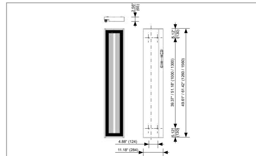
Exterior and mounting dimensions of the VAO PM. All data in Inches (mm).
