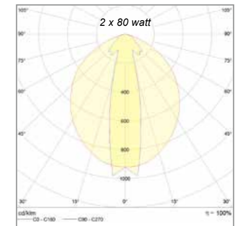
Light distribution curve of LEDMRO (LED-MultiReflexOptic). This chart shows the light distribution curve of an LEDMRO with 2 x 80 watt.
