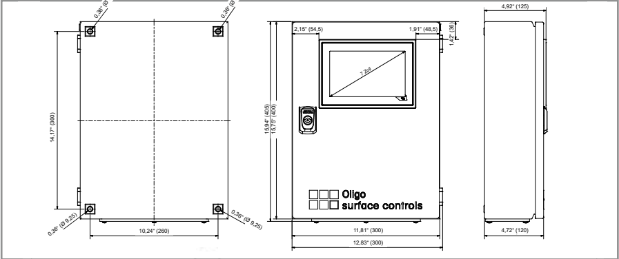
External and mounting dimensions of the HAFST eta7 . All data in Inch (mm).
